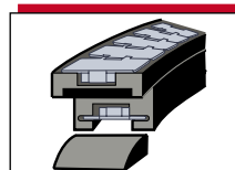
Series COMBI - Page 26 Magnetic corner tracks for chains Series 881 M-880 MG.
