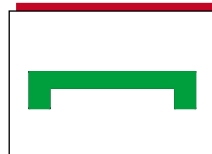
Part. 362 - Page 10 Chain guide profile. Multiple strands K82,5 / pitch 85
