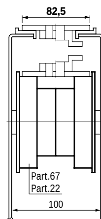
Fig. 68 - Chain width 82,5 mm (K 325) / Pitch 88 mm
