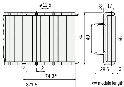
Sideflexing
