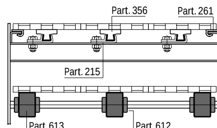
Fig. 59/a - Example of assembly of Part. 613 with MatTop® conveyors
