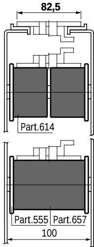
Fig. 56 - Chain width 82,5 mm (K 325) / Pitch 88 mm
