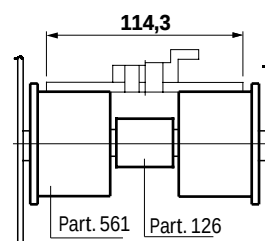
Fig. 51 - Chain width 82,5 mm (K 325) / Pitch 88 mm
