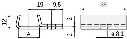
■ Guide rail clamp
