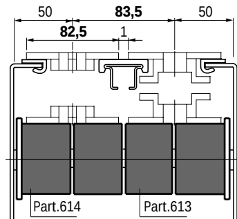
Fig. 59 - Chain width 114,3 mm (K 450) / Pitch 120 mm See fig. 65 page 37
