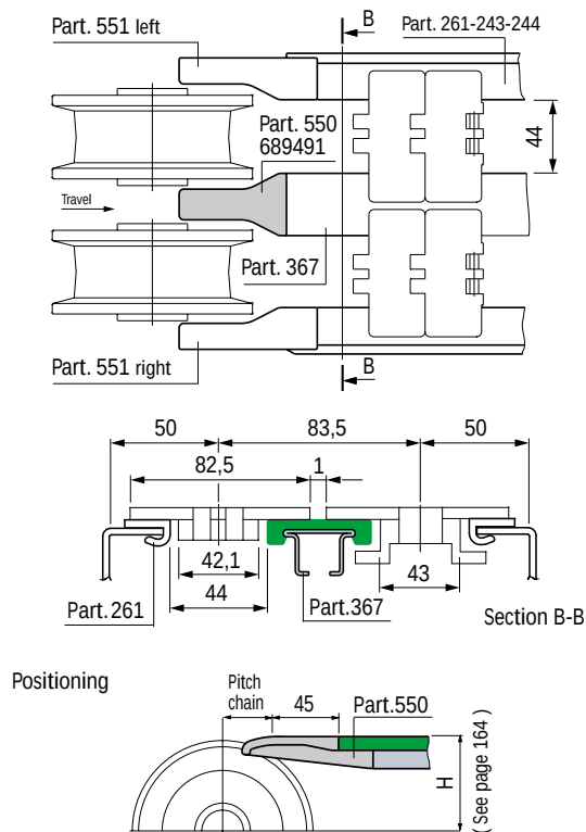
• Fig. 26 - Example of application of Part. 550, in multiple strand conveyor / Chain width 82,5 mm (K325) / Pitch 83,5 mm.
