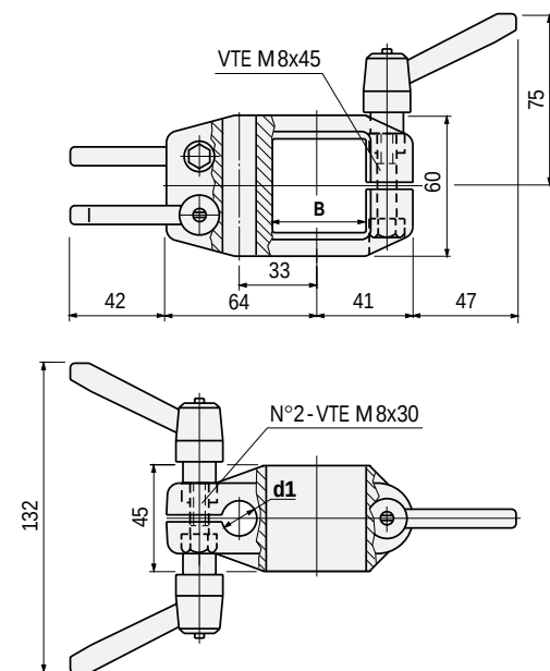
Square bore
