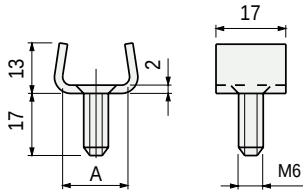
■ Guide rail clamp
