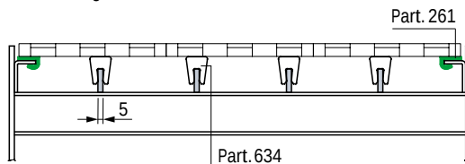
Fig. 16/a - Parallel wear strips. Recommended with medium-light loads.
