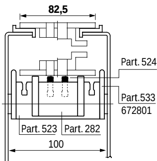
Fig. 72 - Chain width 82,5 mm (K 325) / Pitch 88 mm
