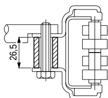
Spacer for double execution guide rail
