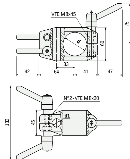
Round bore
