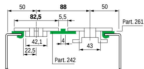
Fig. 14 - Chain width 82,5 mm (K 325) / Pitch 88 mm
