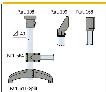
For square tubes 40x40
