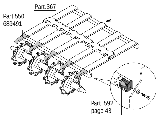
• Fig. 27 - Example of use of Part. 550 in a MatTop® conveyor.
