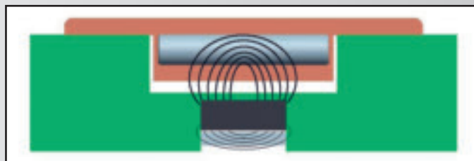
USUAL MAGNETIC CURVE WITH ONLY 1 MAGNET
