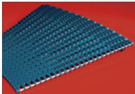
RADIUS 1285 REINFORCED OUTER AND TIGHT FIT INNER MODULES
